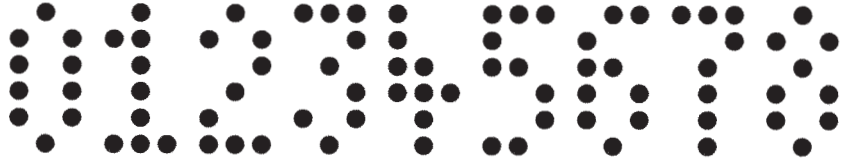
20 mm condensed, matrix 3 x 6, pin Ø 2.3 mm
